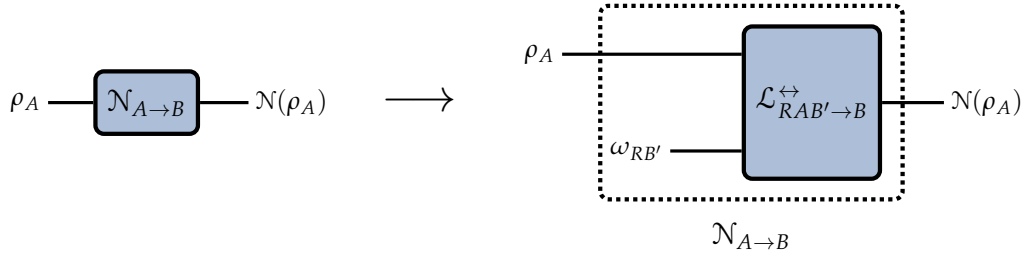
FIGURE 4.8: Depiction of an LOCC-simulable channel \mathcal{N}_{A \rightarrow B} with associated resource state \omega_{RB'} . The channel \mathcal{N}_{A \rightarrow B} can be realized via the LOCC channel \mathcal{L}_{RAB' \rightarrow B}^{\leftrightarrow} and the resource state \omega_{RB'} , for some auxiliary system R . The LOCC channel \mathcal{L}_{RAB' \rightarrow B}^{\leftrightarrow} could in principle consist of a sequence of several rounds of one-way LOCC channels, as depicted in Figure 4.7.
