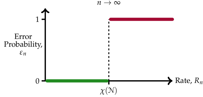
FIGURE 12.5: The error probability \varepsilon_n as a function of the rate R_n for classical communication over a quantum channel \mathcal{N} for which the sandwiched Rényi Holevo information \widetilde{\chi}_\alpha(\mathcal{N}) is additive. As n \rightarrow \infty , for every rate below the Holevo information \chi(\mathcal{N}) , there exists a sequence of protocols with error probability converging to zero. For every rate above the Holevo information \chi(\mathcal{N}) , the error probability converges to one for all possible protocols.
