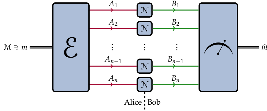
FIGURE 12.3: The most general classical communication protocol over a multiple number n \geq 1 uses of a quantum channel \mathcal{N} . Alice, who wishes to send a message m selected from a set \mathcal{M} , first encodes the message into a quantum state on n quantum systems using a classical–quantum encoding channel \mathcal{E} . She then sends each quantum system through the channel \mathcal{N} . After Bob receives the systems, he performs a collective measurement on them, using the outcome of the measurement to give an estimate \hat{m} of the message m sent to him by Alice.
