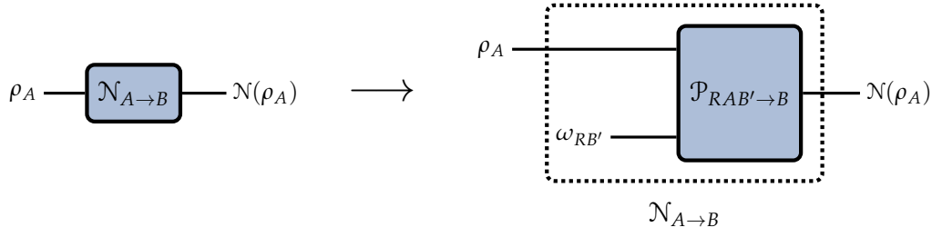
FIGURE 4.9: Depiction of a PPT-simulable channel \mathcal{N}_{A \rightarrow B} with associated resource state \omega_{RB'} . The channel \mathcal{N}_{A \rightarrow B} can be realized via the completely PPT-preserving channel \mathcal{P}_{RAB' \rightarrow B} and the resource state \omega_{RB'} , for some auxiliary system R .
