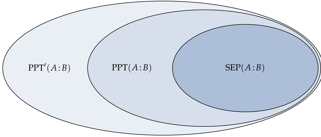
FIGURE 9.2: The set \text{SEP}(A:B) of separable states acting on the Hilbert space \mathcal{H}_{AB} is contained in the set \text{PPT}(A:B) of positive partial transpose (PPT) states, which in turn is contained in the set \text{PPT}'(A:B) of operators defined in (9.1.144). The sets PPT and \text{PPT}' are relaxations of the set of separable states that can be easily characterized in terms of semi-definite constraints.
