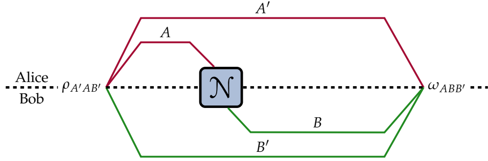
FIGURE 10.1: Starting from a state \rho_{A'AB'} , Alice sends the system A through the channel \mathcal{N}_{A \rightarrow B} to Bob, resulting in the state \omega_{ABB'} = \mathcal{N}_{A \rightarrow B}(\rho_{A'AB'}) . The difference between the final and initial entanglement (as quantified by an entanglement measure for states), optimized over all initial states \rho_{A'AB'} , is equal to the amortized entanglement of \mathcal{N} ; see Definition 10.3.
