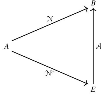
(b) \mathcal{N} anti-degradable.
