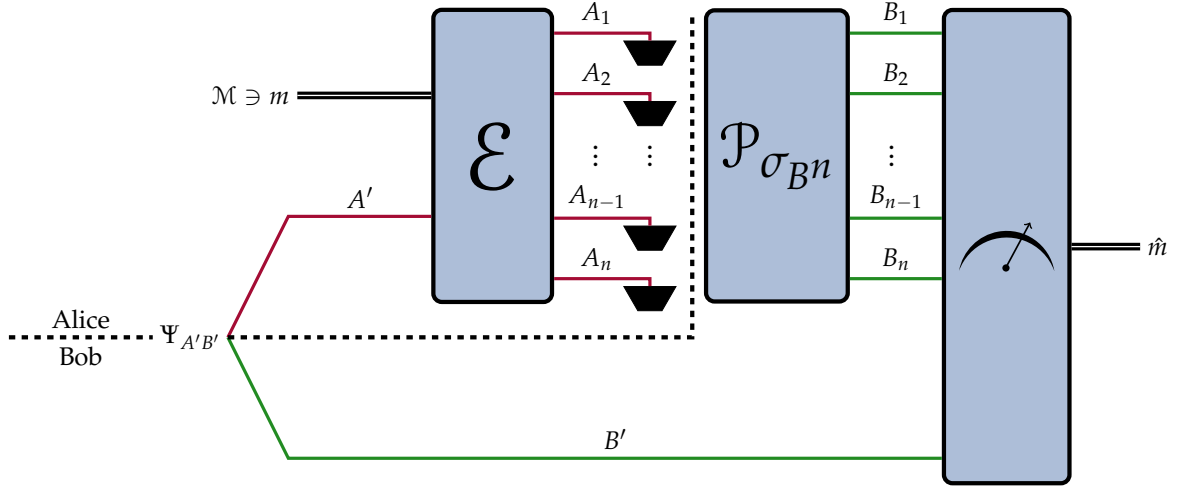
FIGURE 11.5: Depiction of a protocol that is useless for entanglement-assisted classical communication in the asymptotic setting. The state encoding the message m via \mathcal{E} is discarded and replaced by an arbitrary (but fixed) state \sigma_{B^n} .
