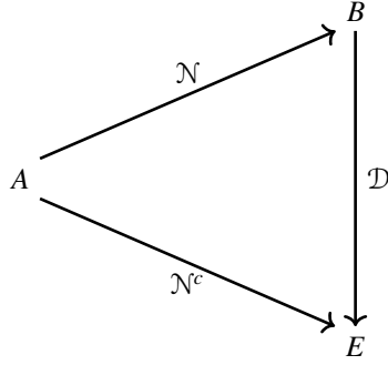
(a) \mathcal{N} degradable.
